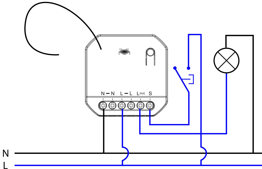
Connection diagram for the 9328
